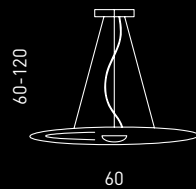
SP 8/321 5 LED 3250 lumen 2700K CE IP20
