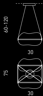
SP 8/324 2 x 14W LED 4000 lumen 3000K CE IP20 ▽
