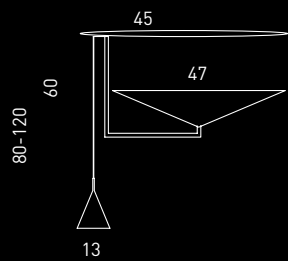
SP 8/320 1 x E27 + GU10 7,2WLED CE IP20
