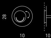
LP 6/321 A LED 650 lumen 2700K CE IP20
