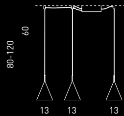
SP 7/320 3 x GU10 7,2W LED CE IP20
