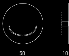
LP 6/321 C 35W 3100 lumen 3000K CE IP20
