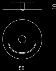
LS 5/321 1 x 12W LED + 35 watt LED 3100 lumen 3000K CE IP20
